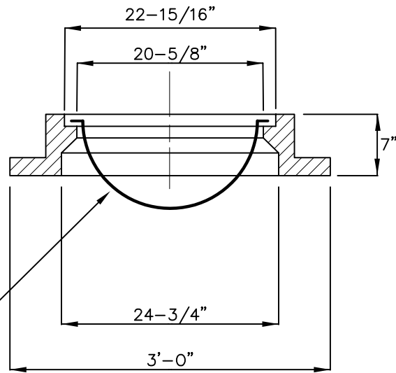
FRAME — SECTION
