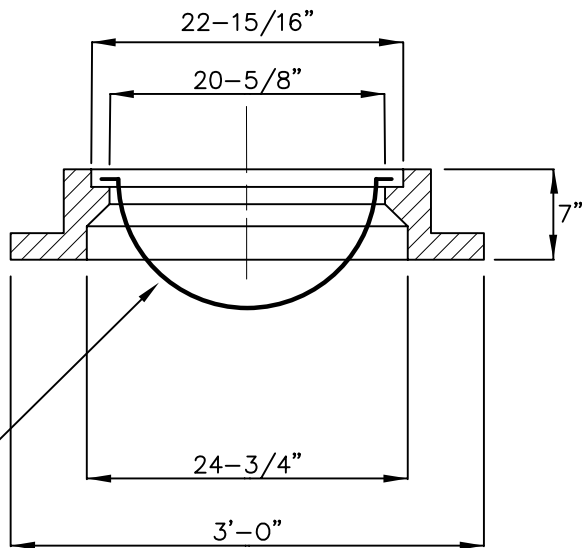
FRAME – SECTION
