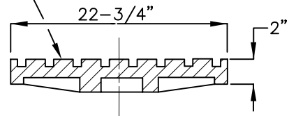
COVER – SECTION
